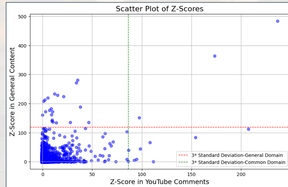
Fig. 5: Scatter Plot of Z-Scores
